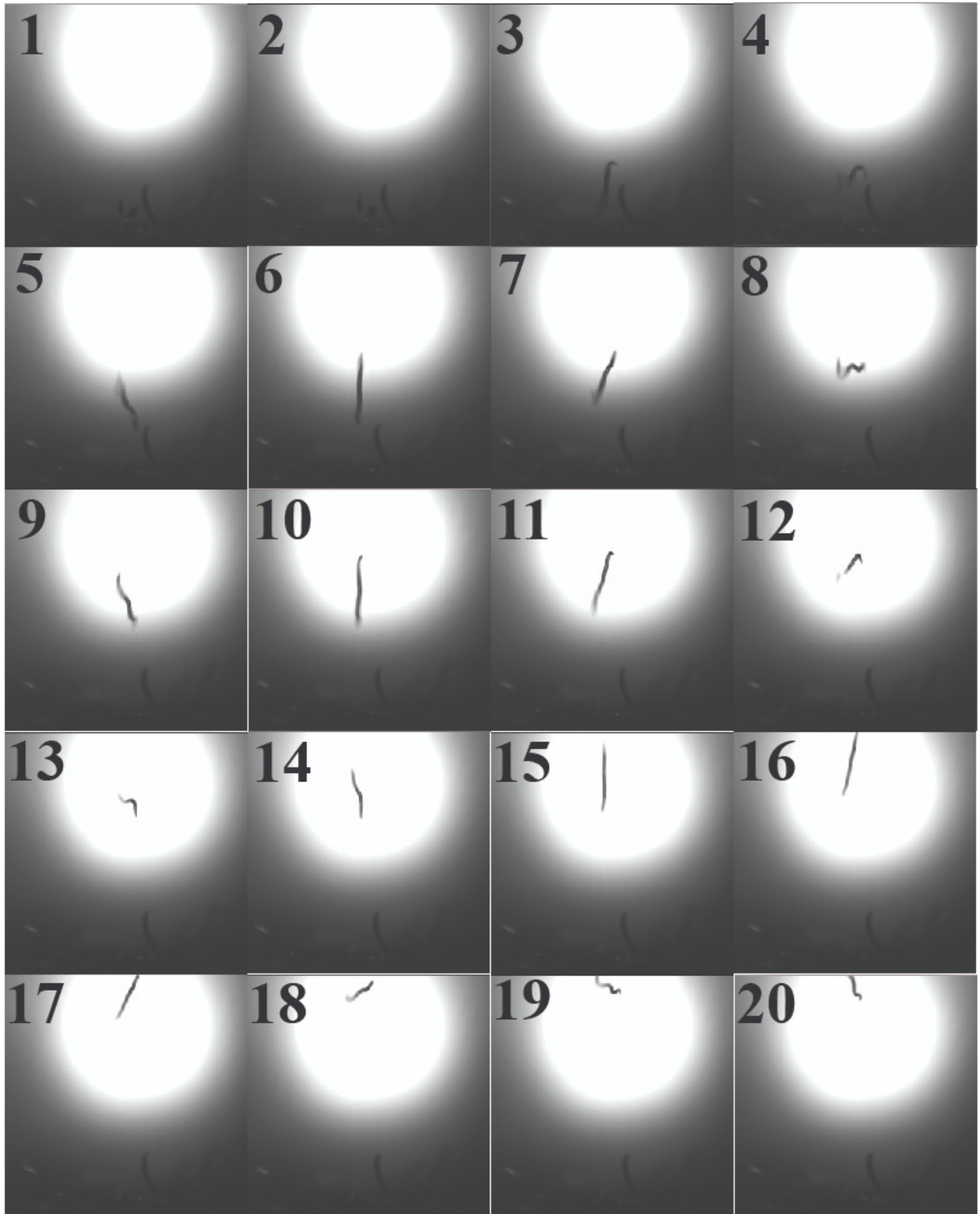
Figure 1: Behavioral sequence for S. carpocapsae IJ jumping (Video 1). The sequence shown, from image 1 to image 20, occurs in approximately 3.88 milliseconds.
